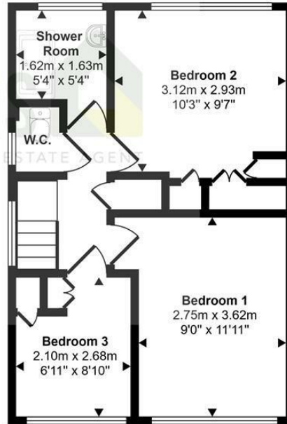
First Floor Approx 37 sq m / 397 sq ft
